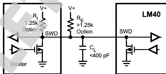
FIGURE 3. SensorPath SWD simplified schematic
